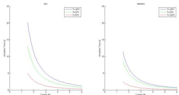
Actuation time at various temperatures Standard Temp Extended Temp
